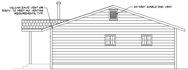
REAR ELEVATION
